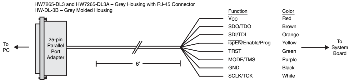
Figure 2. ispDOWNLOAD Cable In-System Programming Interface for the PC 1
